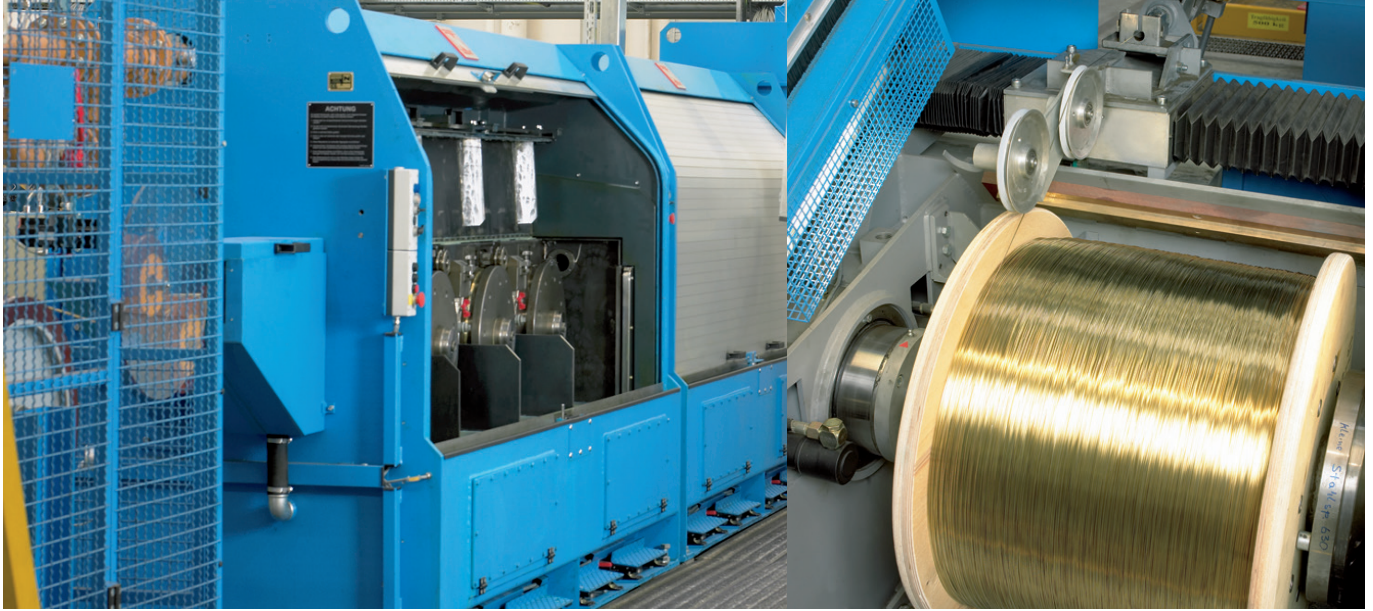
With modern machine technology using high-performance lubricants, the wire is drawn to diameters of minimum 0.3 mm.
